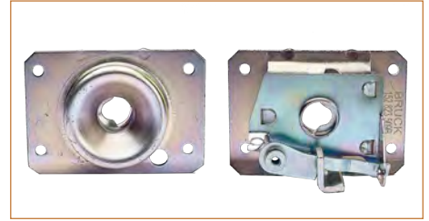
CHAPA COFRE 152823509B CHAPA COFRE SEDAN (1978-2003) 1.6 / (INFERIOR DELANTERA)
