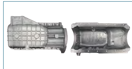
CARTER ACEITE XS6E6675B1G
